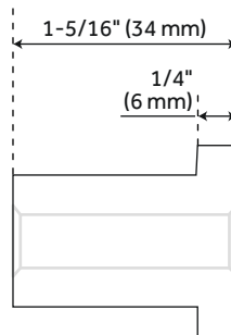
Flat Rail Spacer
