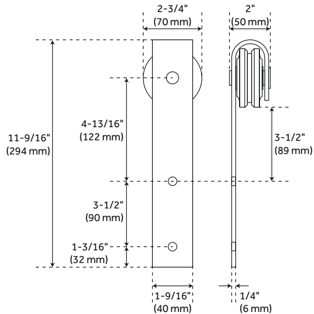
Bent Strap Hanger - Standard Wheel
