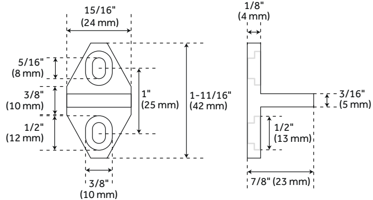
Mortise Floor Guide
