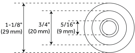
Flat Rail Spacer
