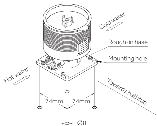
Rough-In Valve Detail
