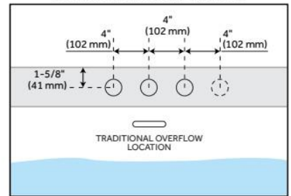
3 & 4 HOLE FAUCET DRILLING
