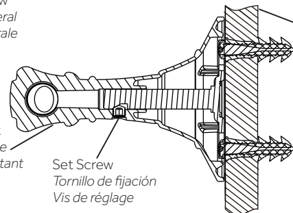
Wall Pared Mur
